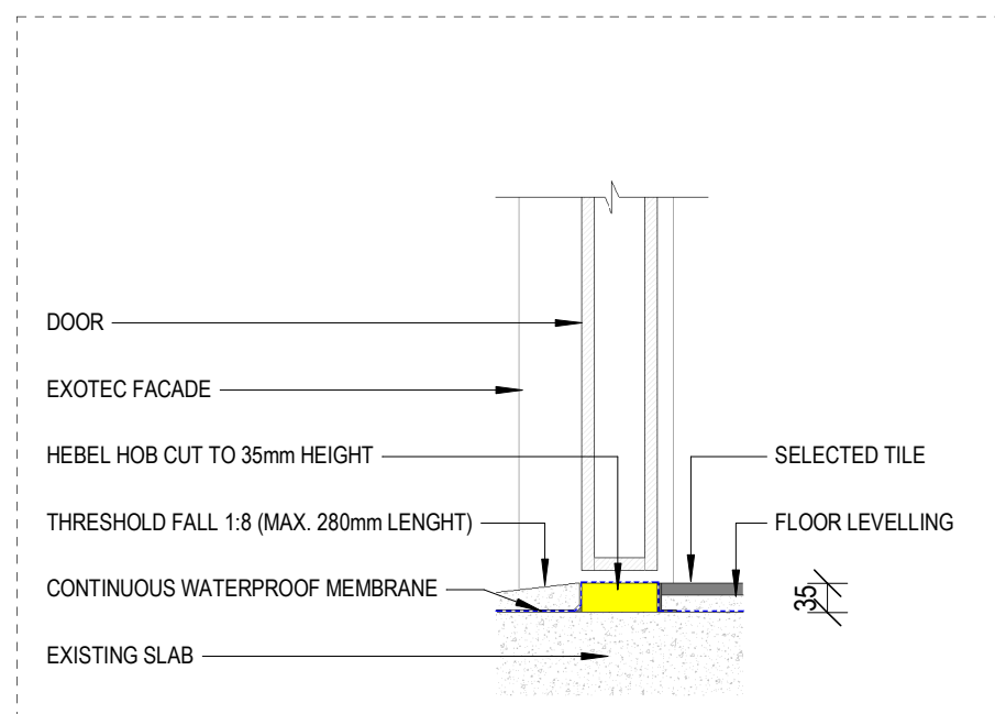
4. TRANSITION BETWEEN EXTERIOR & WET AREA WITH DOOR
