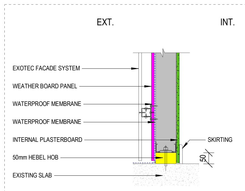
1. TRANSITION BETWEEN EXTERIOR & DRY AREA
