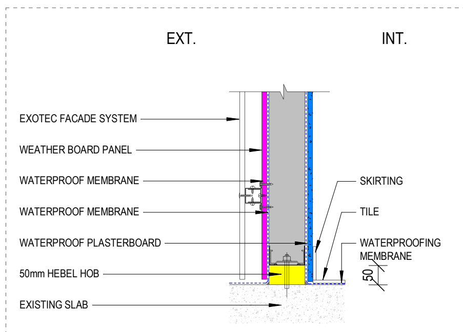
2. TRANSITION BETWEEN EXTERIOR & WET AREA
