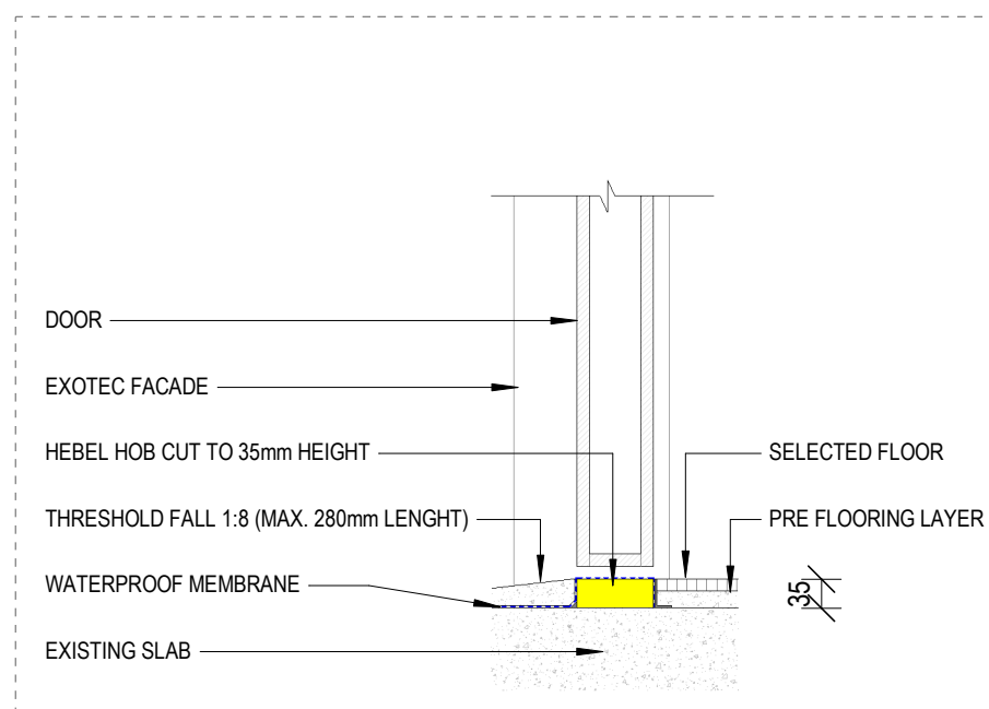
3. TRANSITION BETWEEN EXTERIOR & DRY AREA WITH DOOR
